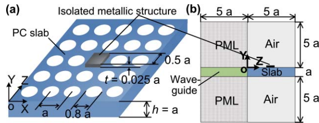
Fig. 1 (a) Schematic of the isolated metal-on-PC slab cavity structure. (b) Cross sectional view (in the Y-Z plane at x = 2.5a ) of the computing region for the 3D PWTMM simulation.
