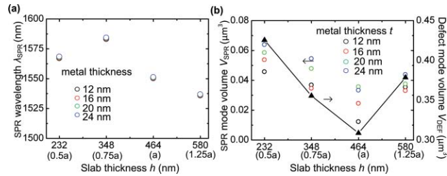
Fig. 4 (a) Dependence of the coupled SPR mode wavelength \lambda_{\text{SPR}} on the slab thickness h for different metal thicknesses t . (b) Left y-axis: dependence of the volume of the coupled SPR mode V_{\text{SPR}} on h for different t . Right y-axis: dependence of the volume of the defect mode of PC cavity V_{\text{DEF}} without the metal ( t = 0 ) on h .
