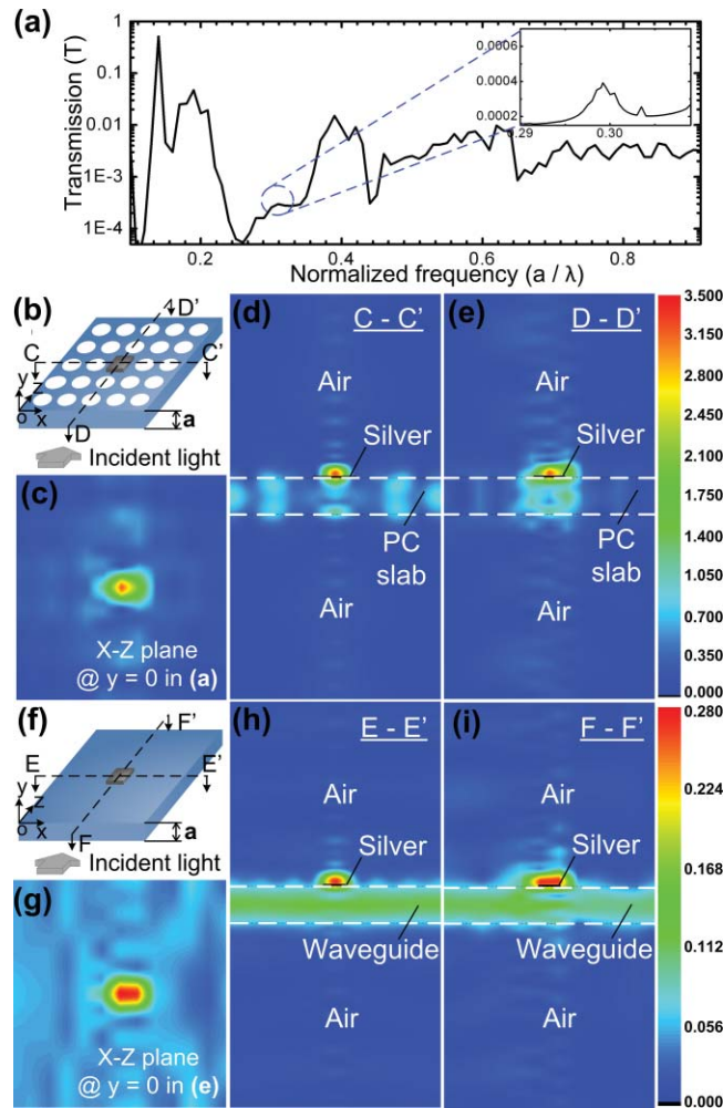
Fig. 3 (a) Transmission spectrum of the isolated metal-on-PC slab cavity structure as a function of the normalized frequency. The inset shows a more detailed spectrum around the defect mode frequency of the cavity. (b) Schematic of the isolated metal-on-PC slab cavity structure for simulation. (c–e) Electric field (amplitude) distributions in the X-Z plane at y = 0 (c), the X-Y plane at the cross-section C-C' (d), and the Y-Z plane at the cross-section D-D' (e) for the structure shown in (b). (f) Schematic of the silicon waveguide–metal counterpart structure for simulation. (g–i) Electric field (amplitude) distributions in the X-Z plane at y = 0 (g), the X-Y plane at the cross section E-E' (h), and the Y-Z plane at the cross-section F-F' (i) for the structure shown in (f).
