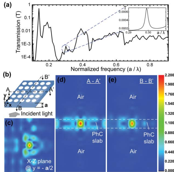
Fig. 2 (a) Transmission spectrum of the PC cavity without the silver structure as a function of the normalized frequency. The inset shows a more detailed spectrum around the defect mode frequency of the cavity. (b) Schematic of the PC cavity used in the simulation. (c–e) Electric field (amplitude) distributions in the X-Z plane at the half height of the slab thickness y = -a/2 (c), in the X-Y plane at the cross-section A-A' (d), and in the Y-Z plane at the cross-section B-B' (e).
